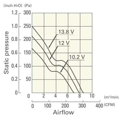
109E5712Y501 With pulse sensor
