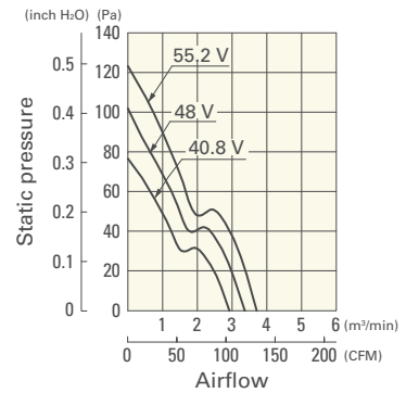
9GL1248M101 With pulse sensor
