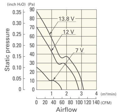
9GL1212H101 With pulse sensor
