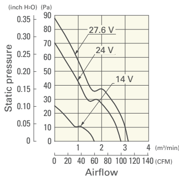
9GL1248G101 With pulse sensor
