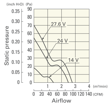
9GL1248E101 With pulse sensor
