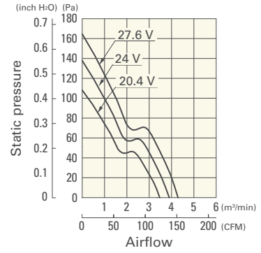
9GL1224F101 With pulse sensor
