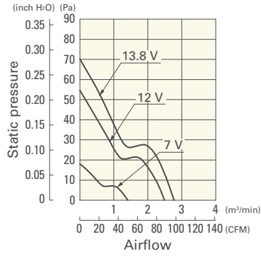
9GL1224E101 With pulse sensor
